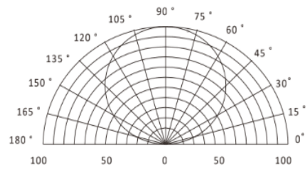
Relative luminous intensity Iv %
